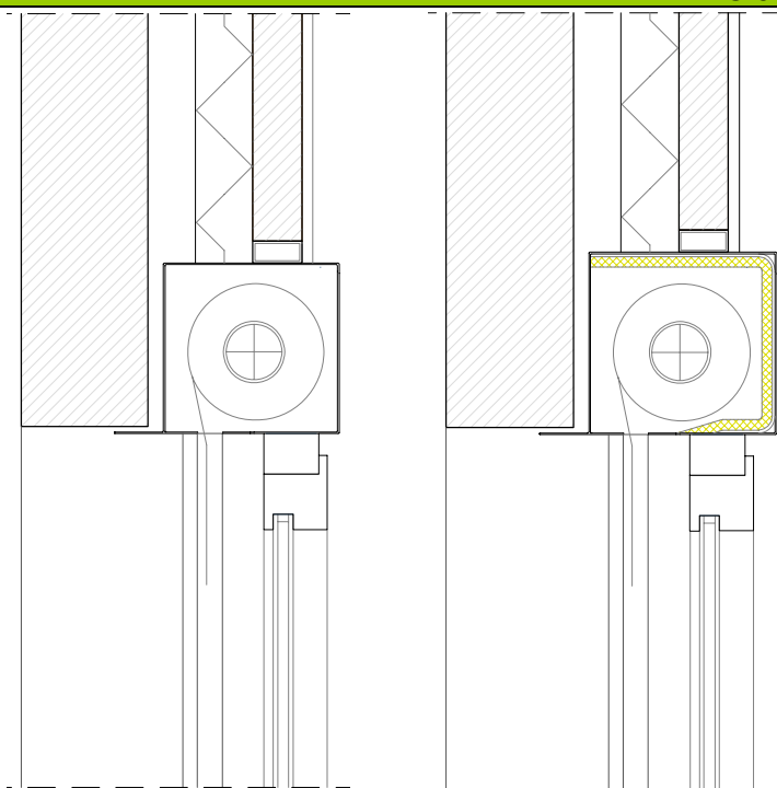
Detalle VC-01.R1
