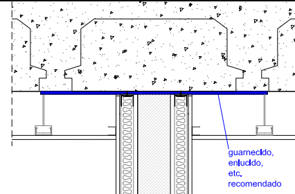
Detalle ESV-01.a.R3
