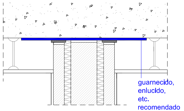
Detalle ESV-02.c-R5
