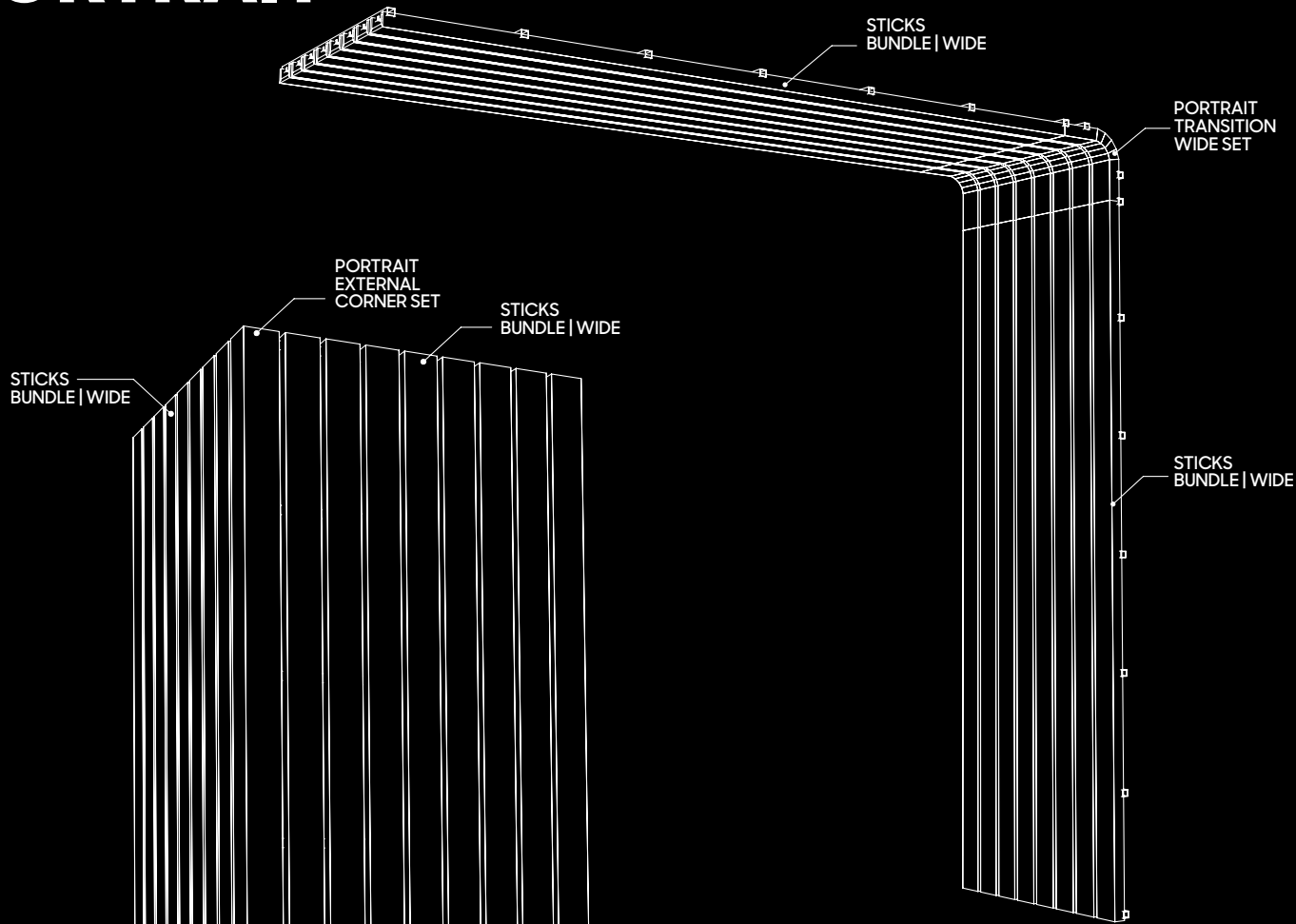
TYPICAL PORTRAIT TRANSITION ASSEMBLY 101mm wide stick profile
